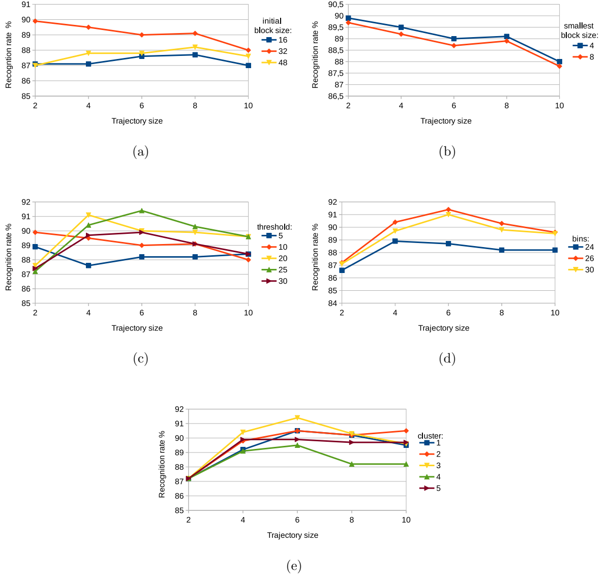
Figure 5.7: Experiments on KTH dataset with third variation
