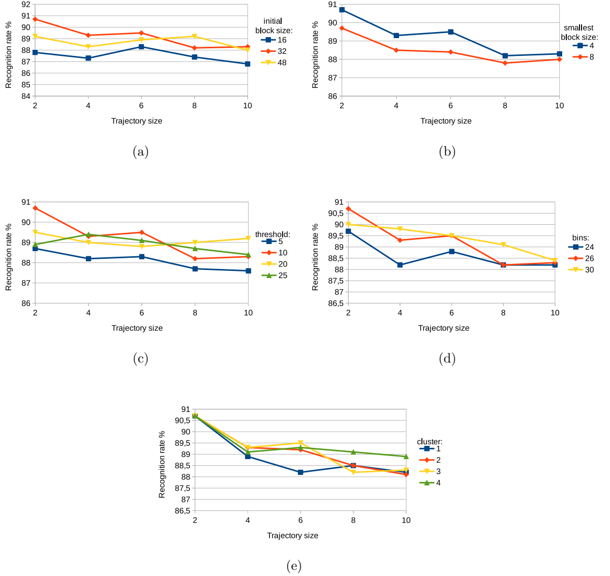
Figure 5.6: Experiments on KTH dataset with second variation
