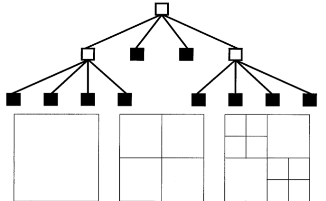
Fig. 2. Quad tree image segmentation (adapted from [13]) yielded by VSBMA. Leaf nodes correspond to blocks of various sizes.
