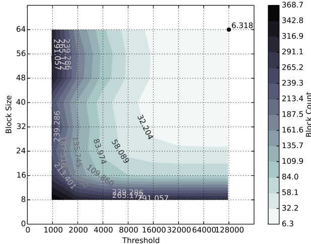
Fig. 13. Contour plot showing block count for each parameter setting. Lighter colors indicate lower number of blocks.
