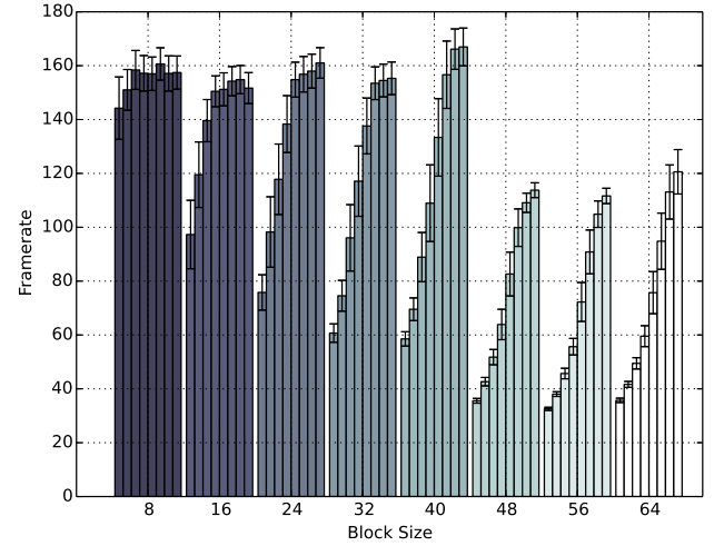
Fig. 10. Bar graph showing running speed for each parameter setting. The bars are grouped by block size and each bar within a group shows the frame rate for a different threshold value. Error bars show the confidence intervals for each case.
