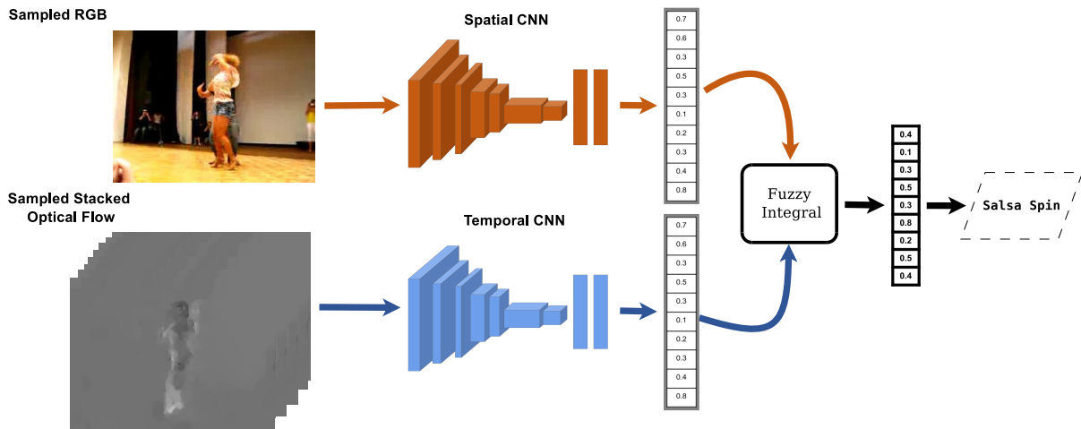
Figure 1: Fuzzy fusion strategy combined with a two-stream architecture for action recognition.
