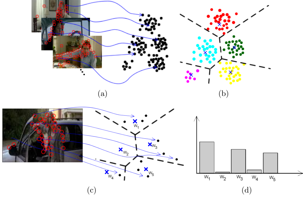
Figure 3.9: Illustration of the BoF steps. (a) all visual words from the training set are gathered together. (b) the visual words are clustered using the k-means algorithm. (c) a new image from the testing set is analyzed and its visual words are matched in the previously generated clusters. (d) the final descriptor is computed based on the frequency of the incidence of each cluster.
